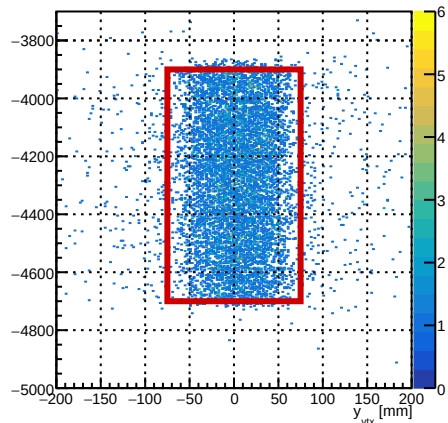
Selected two-track reconstructed vertex
