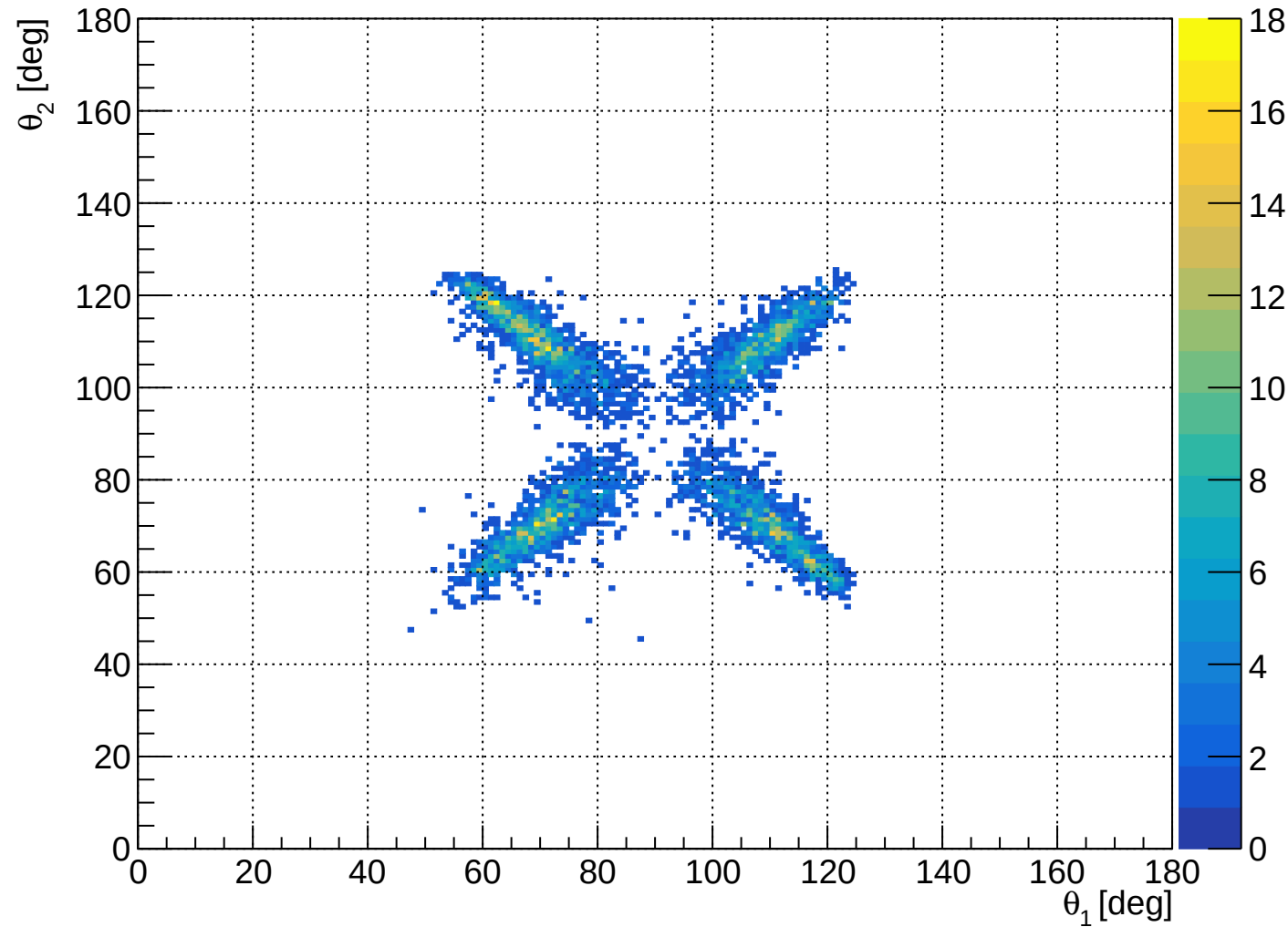
TEST: minimum- |\Delta t| shared ST_Foils momentum polar angles
