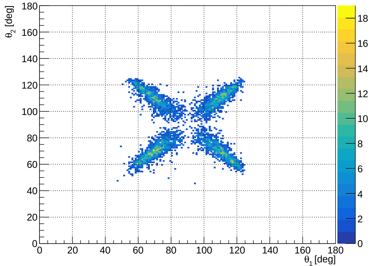
Space-selected shared ST_Foils momentum polar angles
