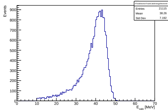
Two-track events: electron 0 calorimeter energy
