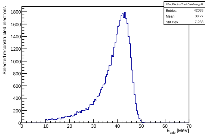
Two-track events: electron calorimeter energy
