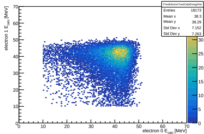
Two-track events: electron calorimeter energy pair
