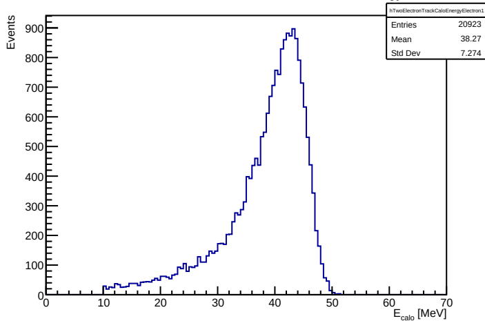
Two-track events: electron 1 calorimeter energy
