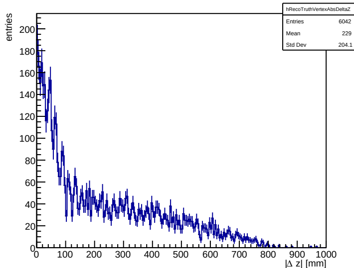
Absolute selected two-track vertex minus truth origin z difference
