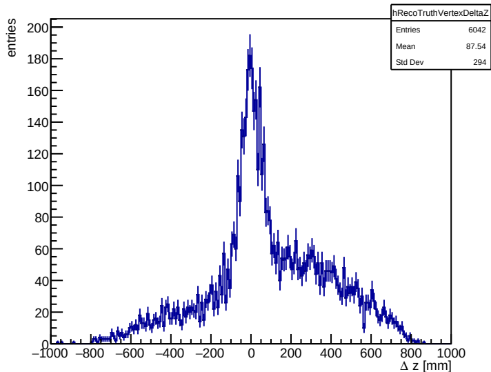
Selected two-track vertex minus truth origin z difference
