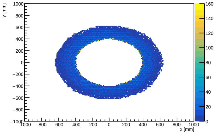
ALL reco e^- tracks: track-calorimeter POCA position
