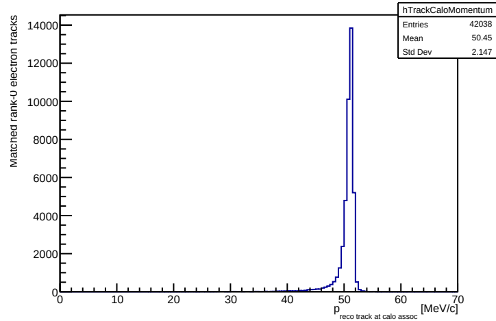
Reconstructed track momentum at track-calor association
