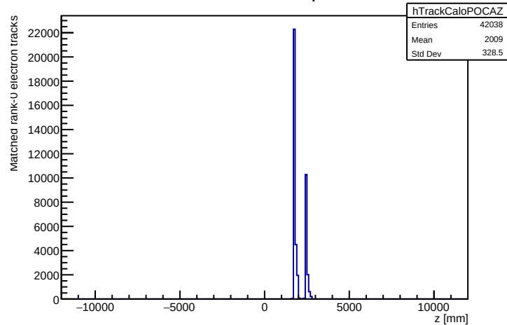
Track-calor POCA z position
