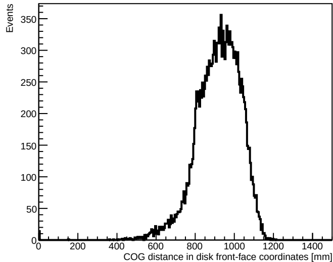
Two-electron events: distance between matched calo cluster COGs
