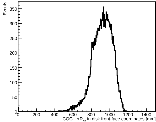
Two-electron events: transverse distance between matched calo cluster COGs
