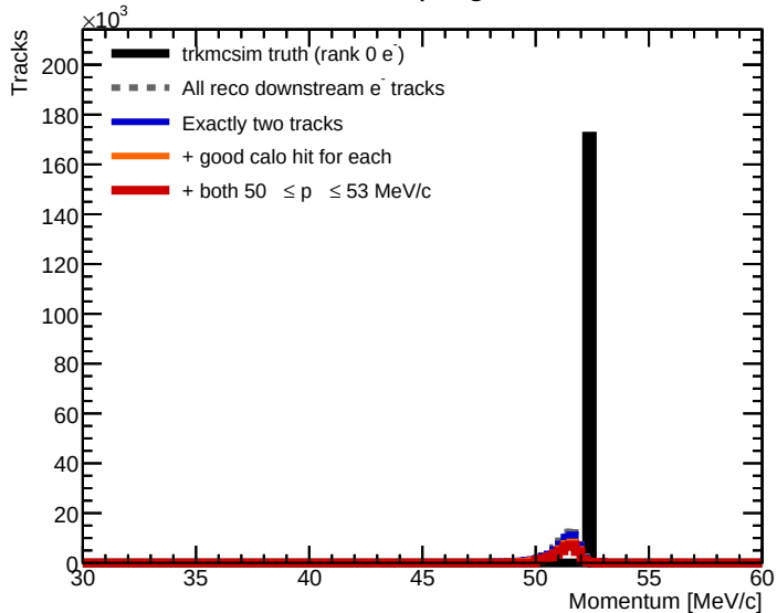
Momentum cut progression
