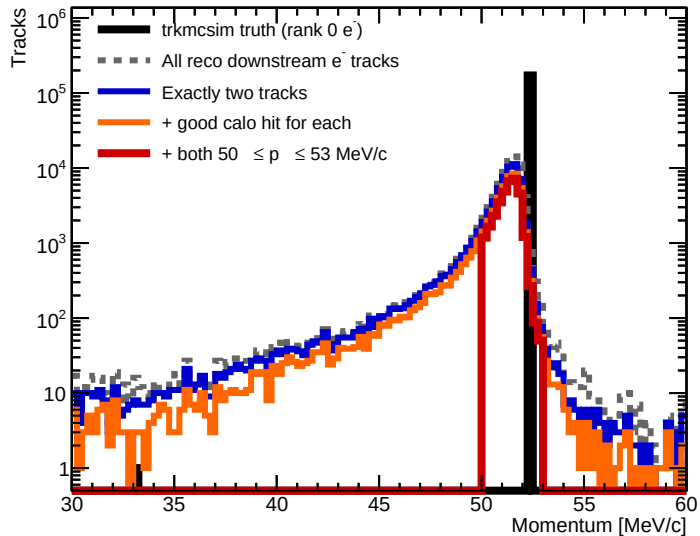
Momentum cut progression (log scale)
