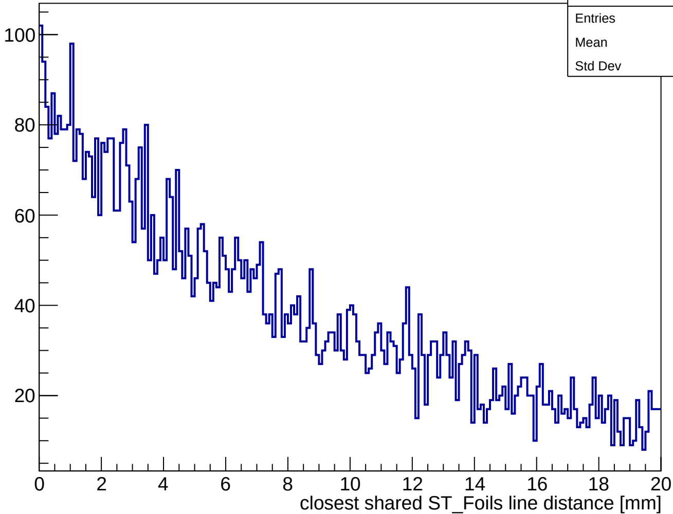
Momentum cut: event-level closest shared ST_Foils line distance
