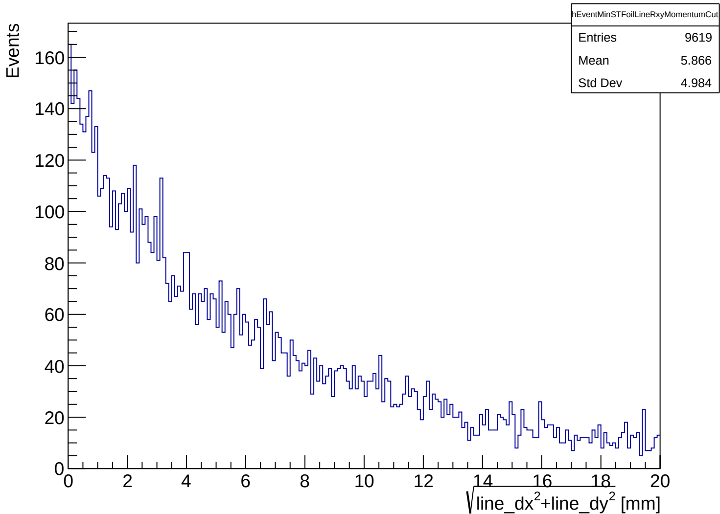
Momentum cut: event-level closest shared ST_Foils transverse separation
