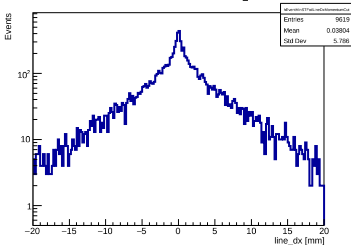
Momentum cut: event-level closest shared ST_Foils line dx
