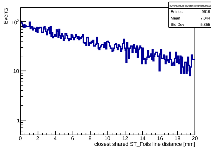
Momentum cut: event-level closest shared ST_Foils line distance
