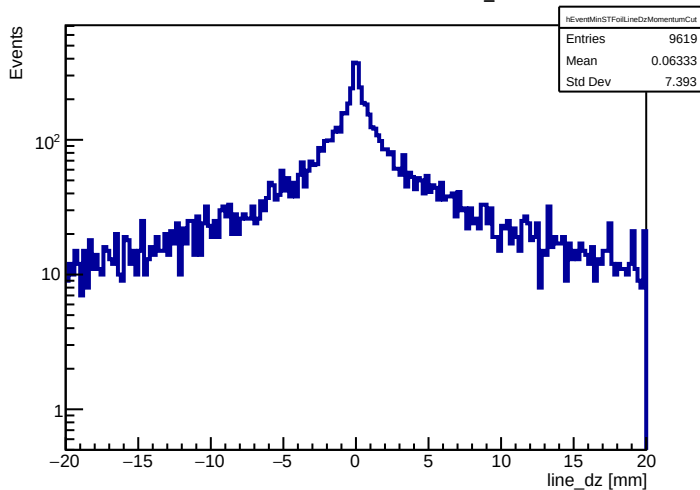
Momentum cut: event-level closest shared ST_Foils line dz
