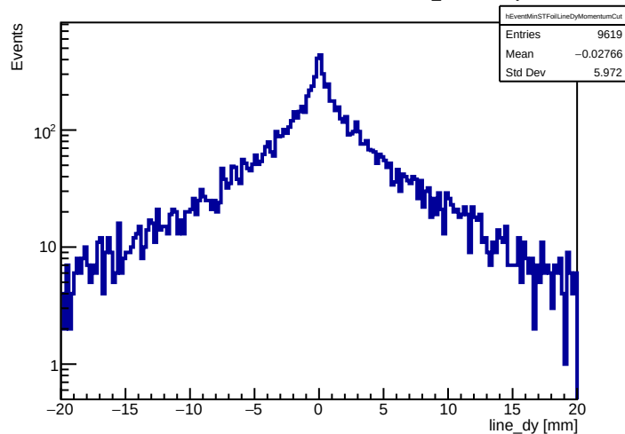
Momentum cut: event-level closest shared ST_Foils line dy
