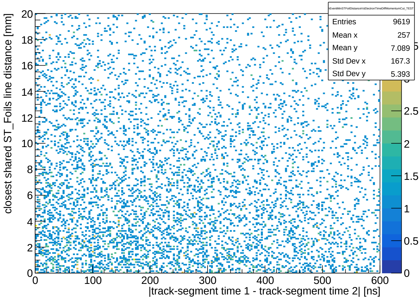
TEST: Momentum cut: event-level closest shared ST_Foils line distance vs absolute shared-foil track-segment time difference
