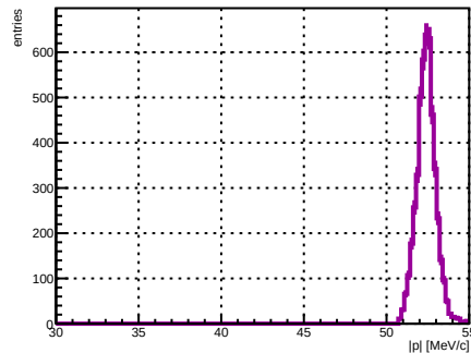
Selected track ST_Foils intersection |p|, foil index 23, N = 4878
