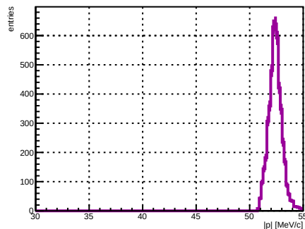
Selected track ST_Foils intersection |p|, foil index 24, N = 4944
