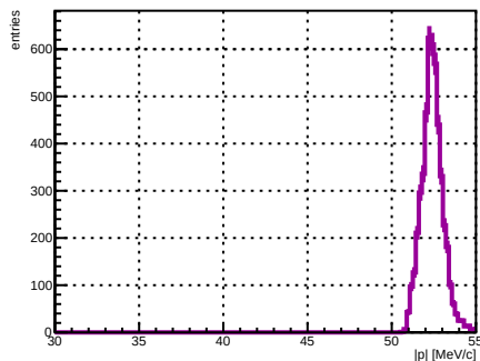
Selected track ST_Foils intersection |p|, foil index 25, N = 4880
