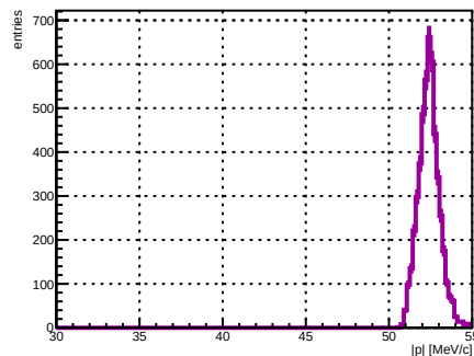
Selected track ST_Foils intersection |p|, foil index 26, N = 5042
