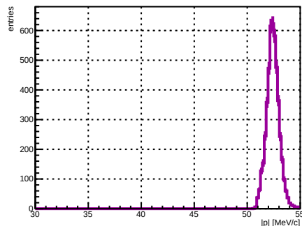
Selected track ST_Foils intersection |p|, foil index 21, N = 4803
