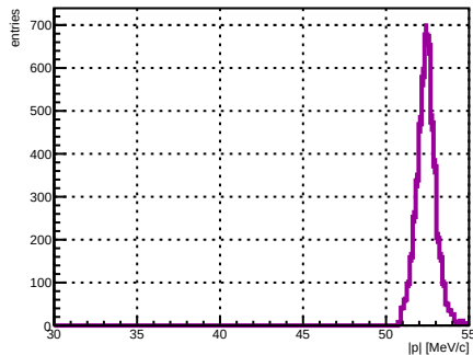
Selected track ST_Foils intersection |p|, foil index 22, N = 4812
