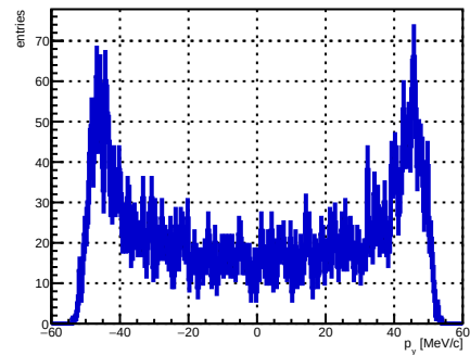
Selected track ST_Foils intersection p_y , foil index 29, N = 4850
