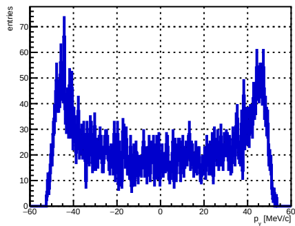
Selected track ST_Foils intersection p_y , foil index 34, N = 4972
