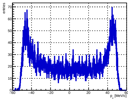
Selected track ST_Foils intersection p_y , foil index 30, N = 4938
