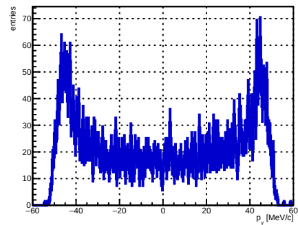
Selected track ST_Foils intersection p_y , foil index 35, N = 4836
