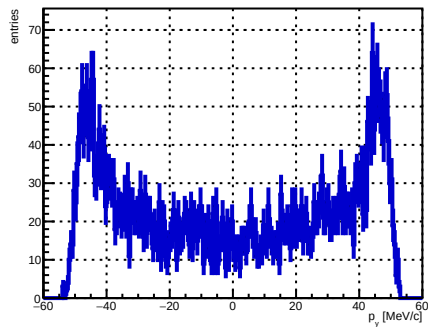
Selected track ST_Foils intersection p_y , foil index 27, N = 4945
