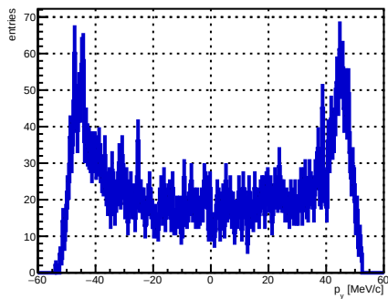
Selected track ST_Foils intersection p_y , foil index 33, N = 4938
