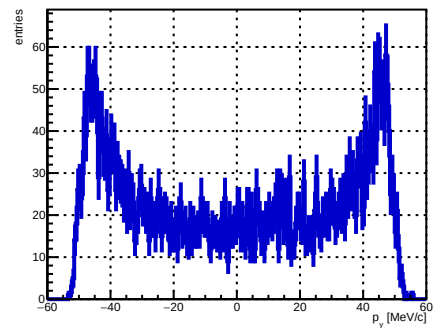
Selected track ST_Foils intersection p_y , foil index 32, N = 4920
