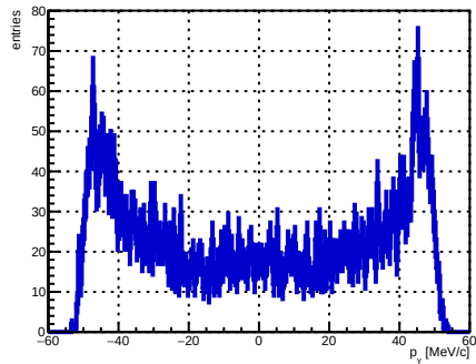
Selected track ST_Foils intersection p_y , foil index 31, N = 4961
