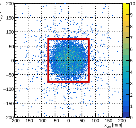
Selected two-track reconstructed vertex
