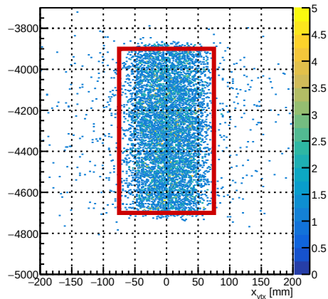
Selected two-track reconstructed vertex
