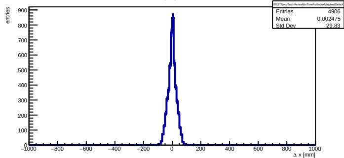
TEST: foil-index matched minimum- |\Delta t| vertex minus truth origin x difference
