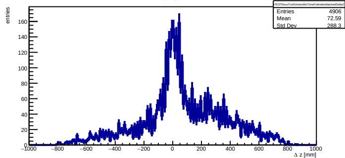
TEST: foil-index matched minimum- |\Delta t| vertex minus truth origin z difference
