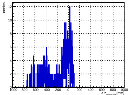
selected foil index 4, N = 150
