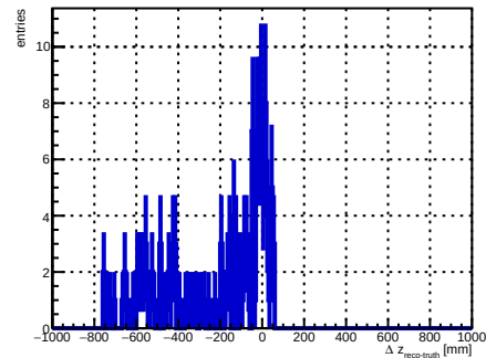
selected foil index 5, N = 161
