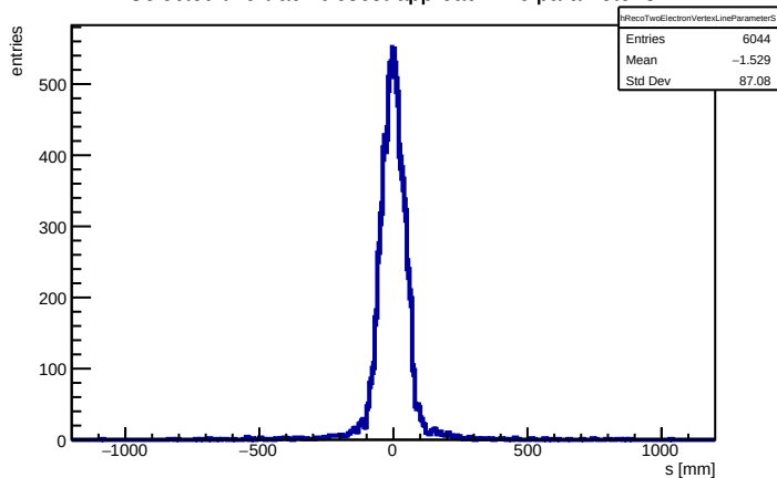
Selected two-track closest-approach parameter s
