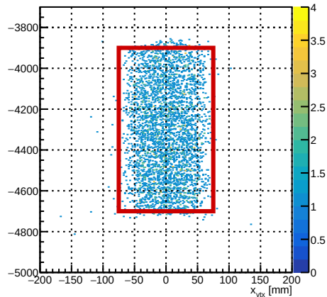
Foil-index matched selected two-track reconstructed vertex
