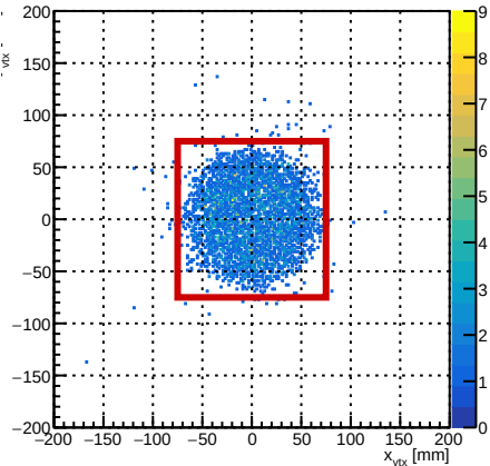
Foil-index matched selected two-track reconstructed vertex
