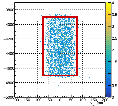
Foil-index matched selected two-track reconstructed vertex
