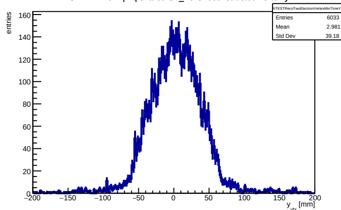
TEST: minimum- |\Delta t| shared ST_Foils reconstructed vertex y
