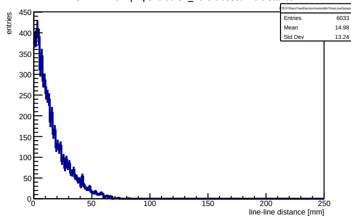
TEST: minimum- |\Delta t| shared ST_Foils closest-line distance
