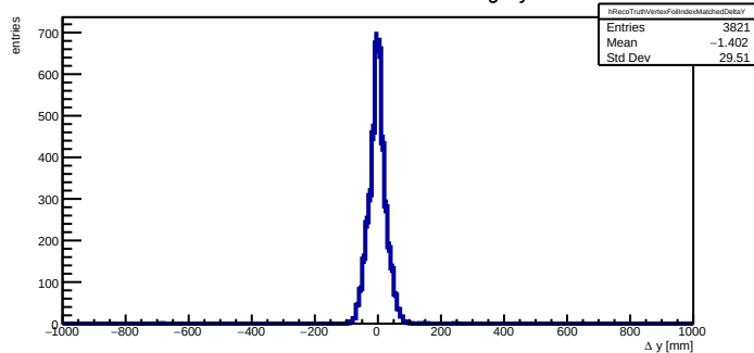
Foil-index matched vertex minus truth origin y difference
