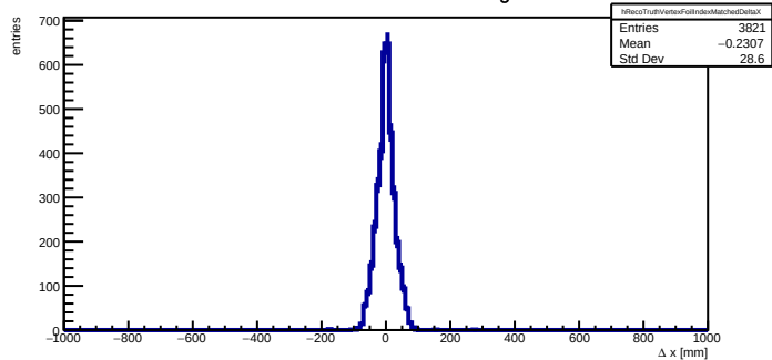
Foil-index matched vertex minus truth origin x difference
