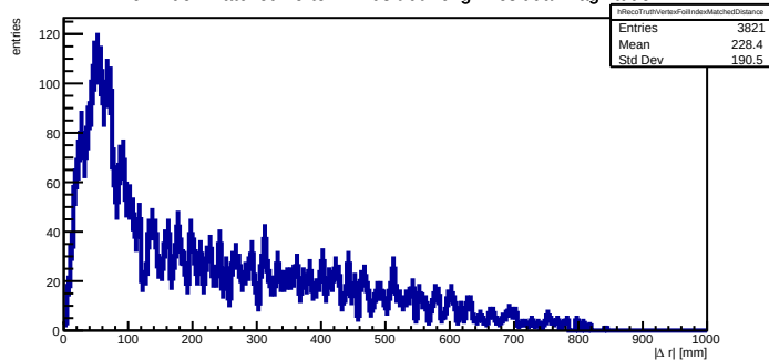
Foil-index matched vertex minus truth origin residual magnitude
