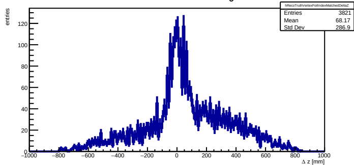
Foil-index matched vertex minus truth origin z difference
