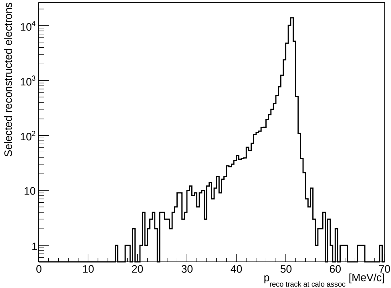
Two-track events: reconstructed track momentum at track-calorimeter association
