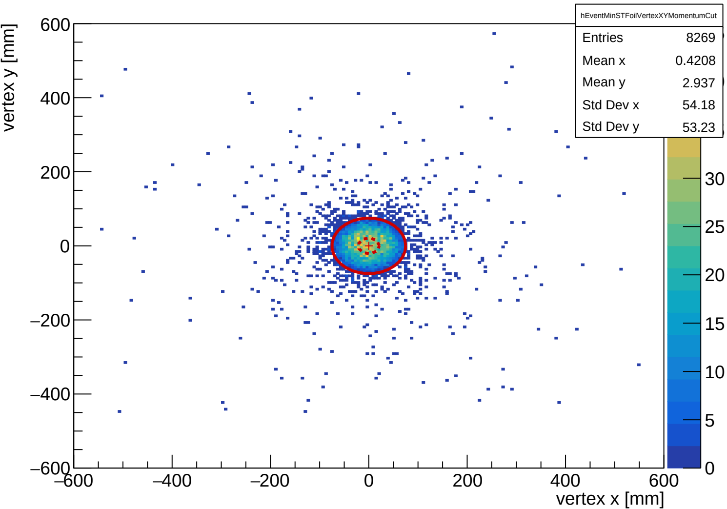
Momentum cut: event-level closest shared ST_Foils midpoint vertex XY
