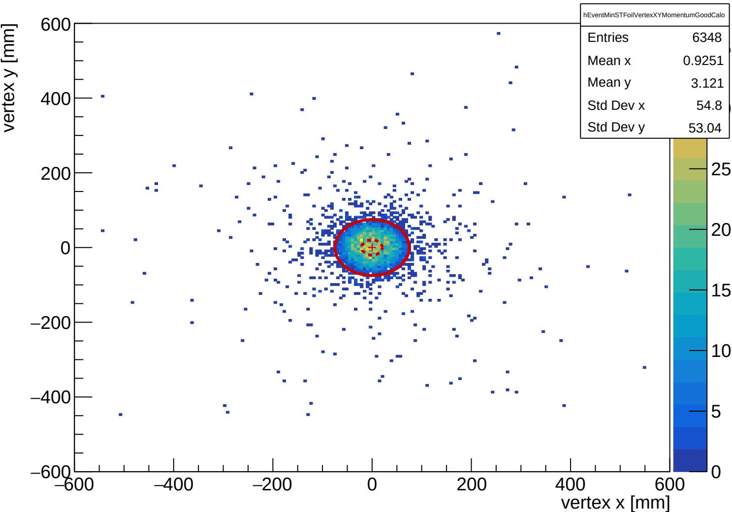
Momentum + good calo: event-level closest shared ST_Foils midpoint vertex XY
