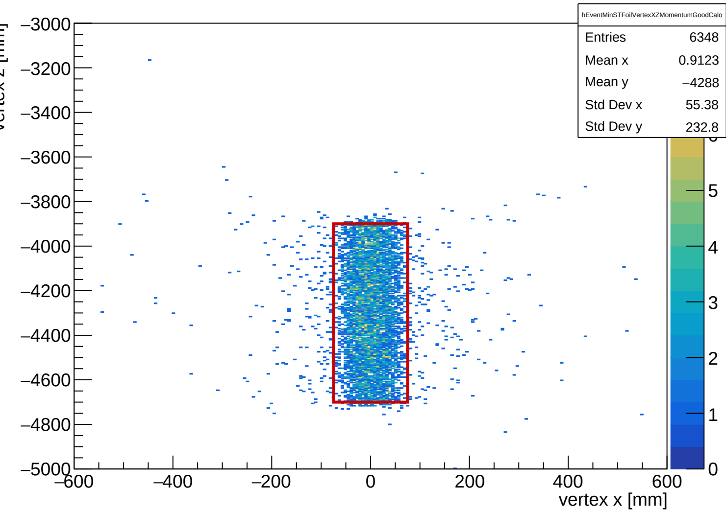
Momentum + good calo: event-level closest shared ST_Foils midpoint vertex XZ
