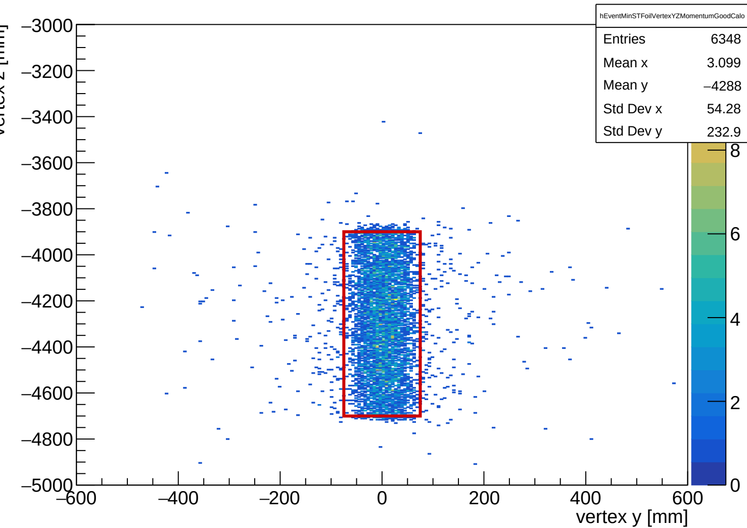
Momentum + good calo: event-level closest shared ST_Foils midpoint vertex YZ
