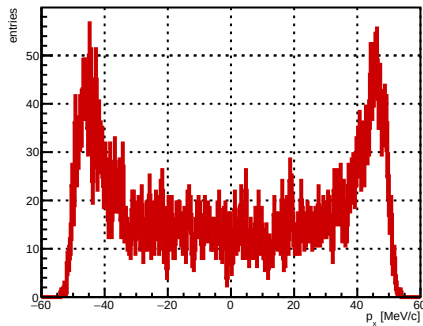
Selected track ST_Foils intersection p_x , foil index 27, N = 3985
