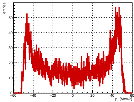
Selected track ST_Foils intersection p_x , foil index 34, N = 3879
