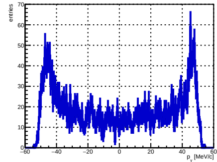
Selected track ST_Foils intersection p_y , foil index 26, N = 4058
