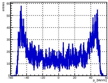
Selected track ST_Foils intersection p_y , foil index 24, N = 3868
