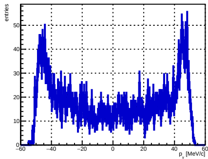
Selected track ST_Foils intersection p_y , foil index 25, N = 3926
