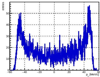
Selected track ST_Foils intersection p_y , foil index 21, N = 3895
