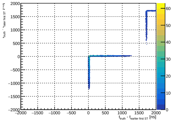
Selected event timing residuals
