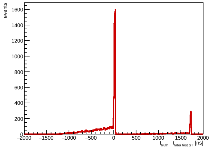
Selected event timing residuals
