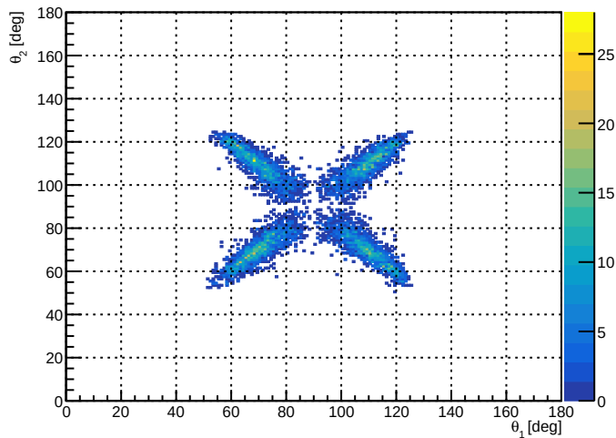
Space-selected shared ST_Foils momentum polar angles
