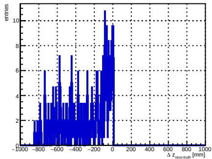
selected foil index 3, N = 198
