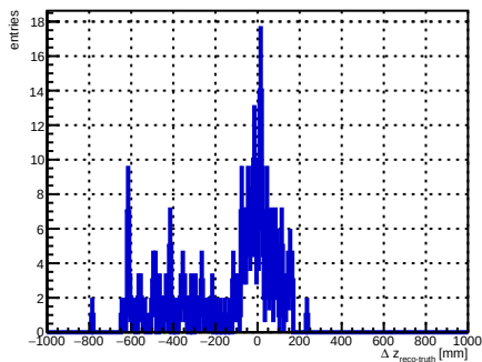
selected foil index 7, N = 204
