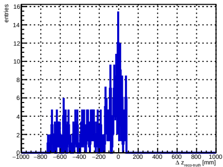
selected foil index 6, N = 216
