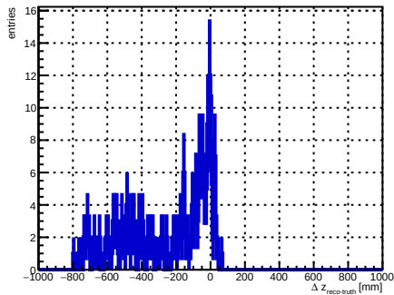
selected foil index 4, N = 190
