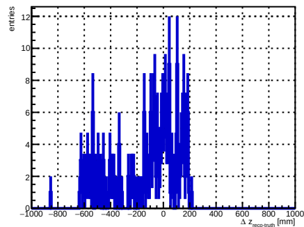
selected foil index 8, N = 211
