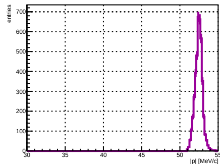
Selected track ST_Foils intersection |p|, foil index 5, N = 4143
