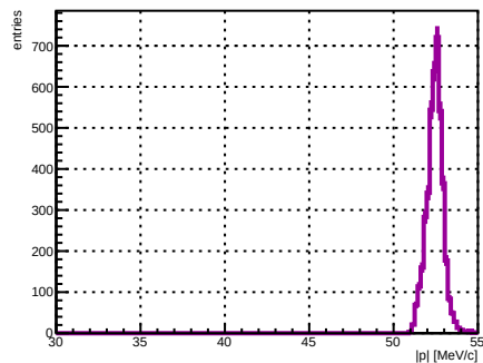
Selected track ST_Foils intersection |p|, foil index 6, N = 4188
