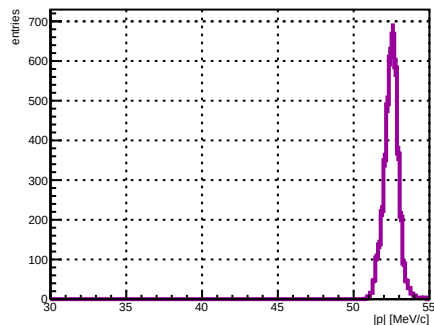
Selected track ST_Foils intersection |p|, foil index 3, N = 4027
