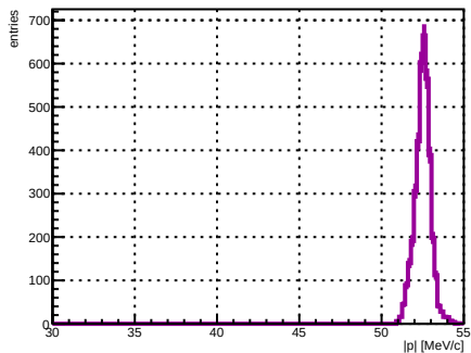
Selected track ST_Foils intersection |p|, foil index 4, N = 4141
