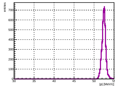
Selected track ST_Foils intersection |p|, foil index 8, N = 4348
