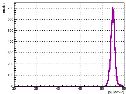
Selected track ST_Foils intersection |p|, foil index 7, N = 4292
