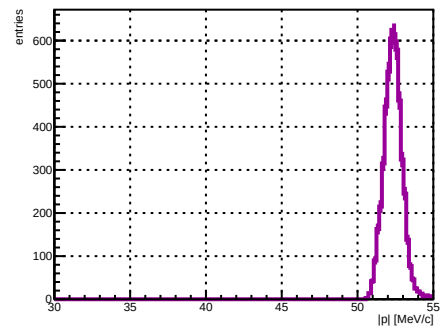
Selected track ST_Foils intersection |p|, foil index 35, N = 4999
