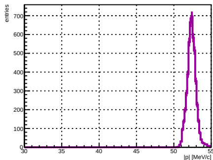
Selected track ST_Foils intersection |p|, foil index 31, N = 5110
