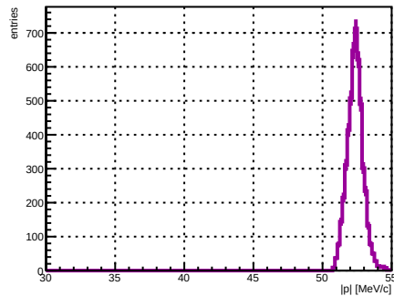
Selected track ST_Foils intersection |p|, foil index 30, N = 5138
