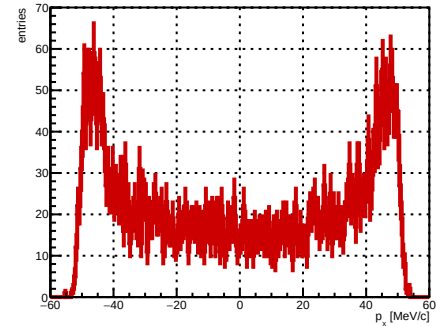
Selected track ST_Foils intersection p_x , foil index 20, N = 4784
