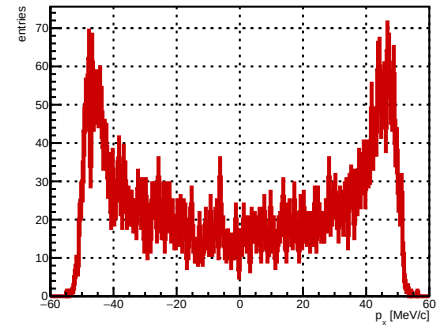
Selected track ST_Foils intersection p_x , foil index 26, N = 5148
