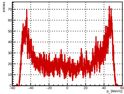
Selected track ST_Foils intersection p_x , foil index 25, N = 5098
