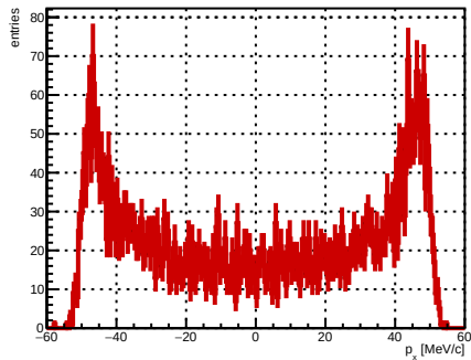
Selected track ST_Foils intersection p_x , foil index 22, N = 5019
