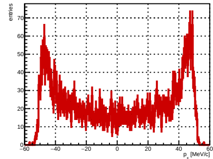
Selected track ST_Foils intersection p_x , foil index 23, N = 4989
