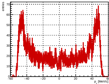
Selected track ST_Foils intersection p_x , foil index 21, N = 4936
