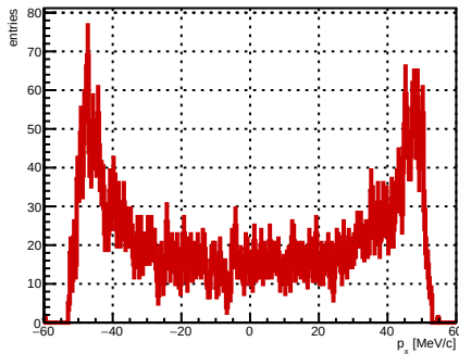
Selected track ST_Foils intersection p_x , foil index 18, N = 4745
