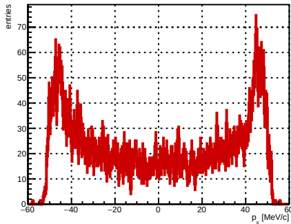
Selected track ST_Foils intersection p_x , foil index 24, N = 4981
