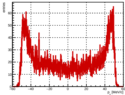
Selected track ST_Foils intersection p_x , foil index 19, N = 4718
