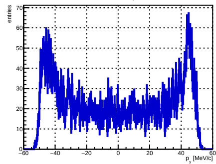
Selected track ST_Foils intersection p_y , foil index 35, N = 4999
