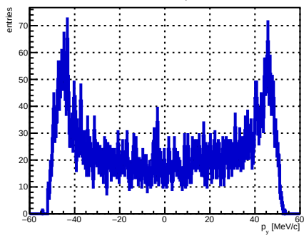
Selected track ST_Foils intersection p_y , foil index 33, N = 5048
