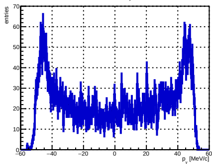
Selected track ST_Foils intersection p_y , foil index 30, N = 5138
