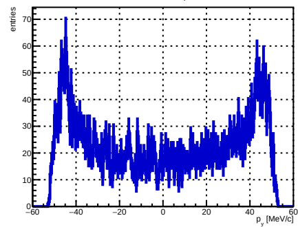
Selected track ST_Foils intersection p_y , foil index 32, N = 4991
