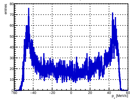
Selected track ST_Foils intersection p_y , foil index 29, N = 5009
