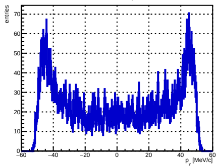
Selected track ST_Foils intersection p_y , foil index 34, N = 5133
