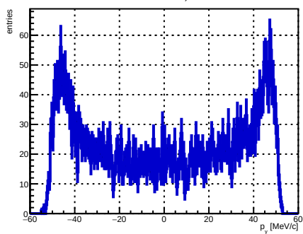
Selected track ST_Foils intersection p_y , foil index 27, N = 5065
