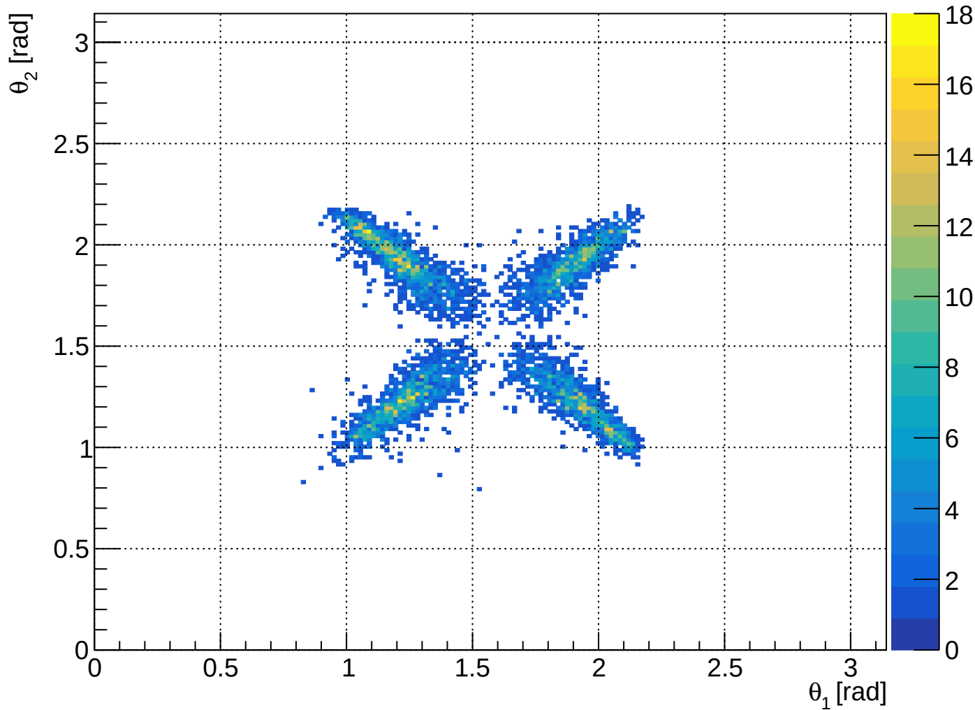
TEST: minimum- |\Delta t| shared ST_Foils momentum polar angles
