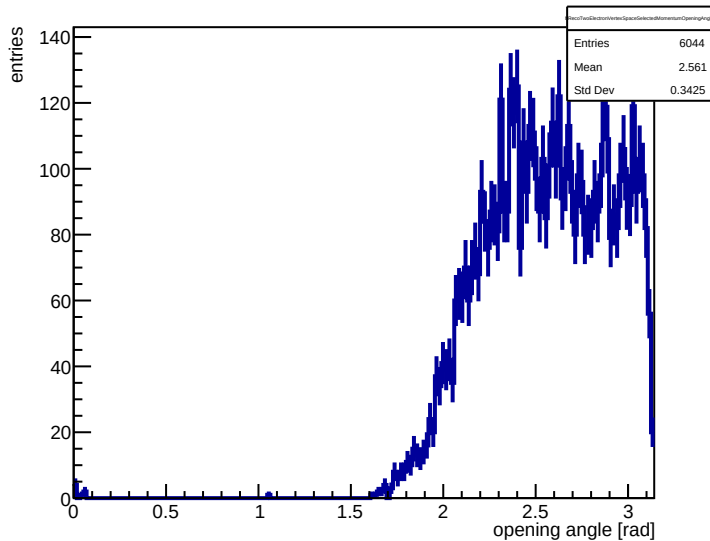
Space-selected shared ST_Foils momentum opening angle
