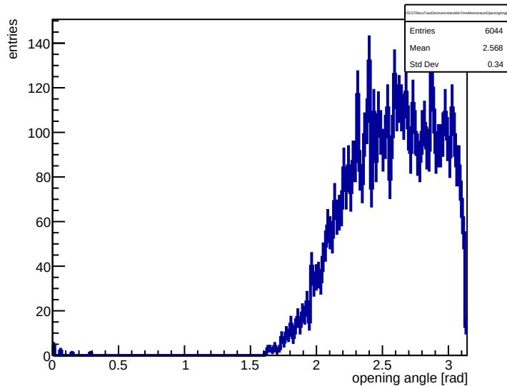
TEST: minimum- |\Delta t| shared ST_Foils momentum opening angle
