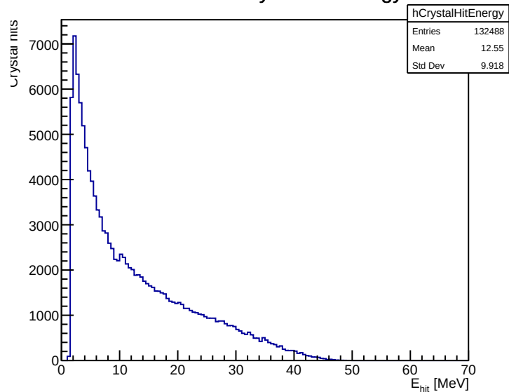
Calorimeter crystal-hit energy
