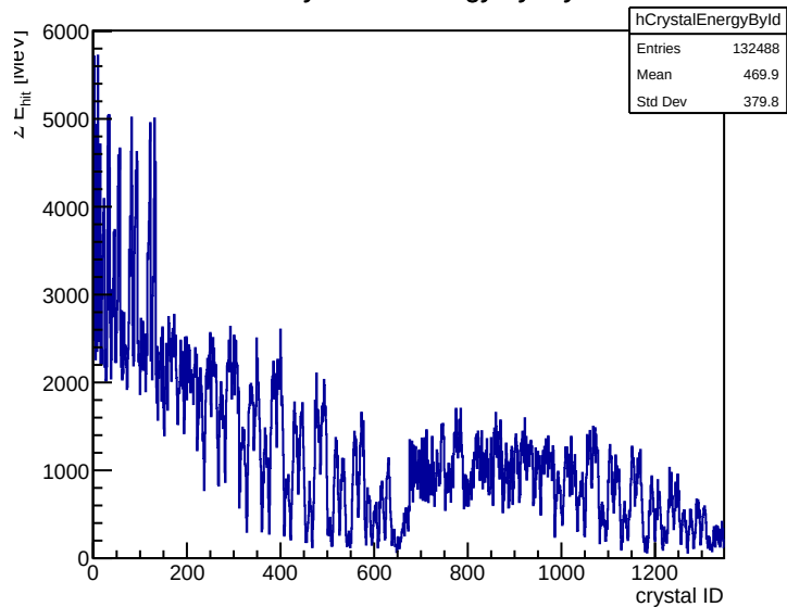
Summed crystal-hit energy by crystal ID
