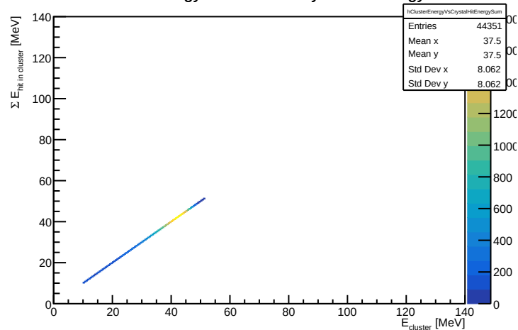
Cluster energy vs summed crystal-hit energy
