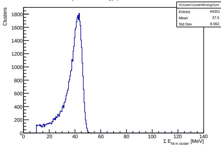
Summed crystal-hit energy per reconstructed cluster
