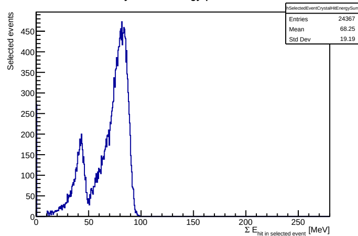
Summed crystal-hit energy per selected event
