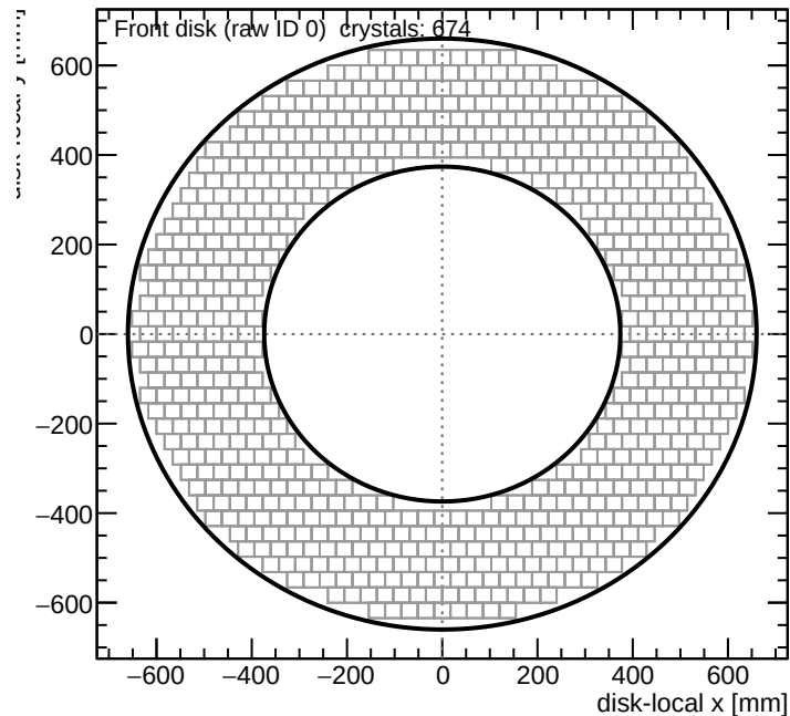
Calorimeter Front disk (raw ID 0)
