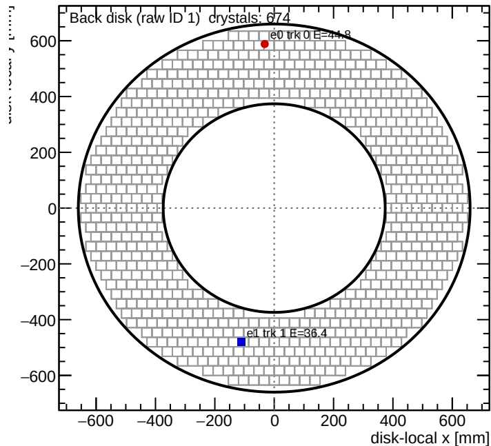
Calorimeter Back disk (raw ID 1)
