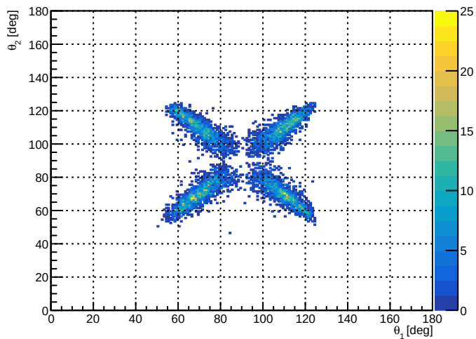
Space-selected shared ST_Foils momentum polar angles
