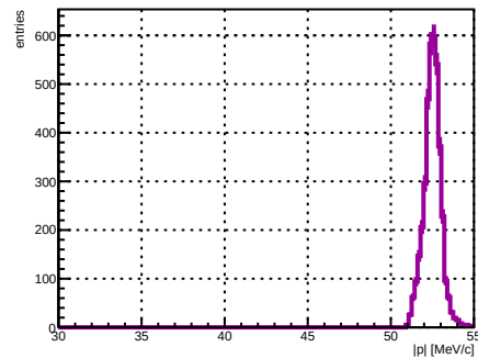
Selected track ST_Foils intersection |p|, foil index 2, N = 3881
