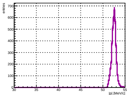
Selected track ST_Foils intersection |p|, foil index 4, N = 4128
