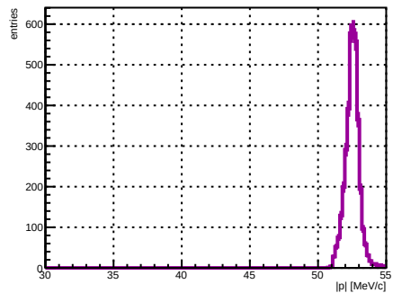
Selected track ST_Foils intersection |p|, foil index 0, N = 3700
