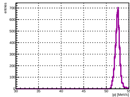
Selected track ST_Foils intersection |p|, foil index 8, N = 4245
