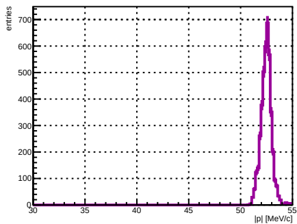
Selected track ST_Foils intersection |p|, foil index 7, N = 4164
