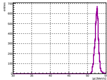
Selected track ST_Foils intersection |p|, foil index 5, N = 4105
