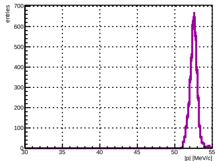
Selected track ST_Foils intersection |p|, foil index 3, N = 4056
