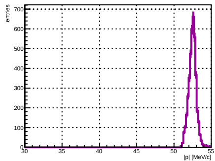
Selected track ST_Foils intersection |p|, foil index 6, N = 4116
