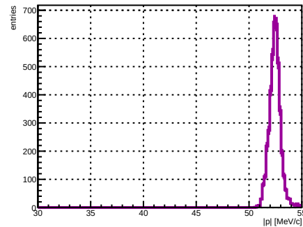
Selected track ST_Foils intersection |p|, foil index 14, N = 4320
