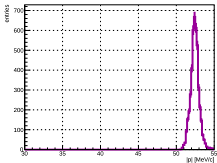
Selected track ST_Foils intersection |p|, foil index 16, N = 4494
