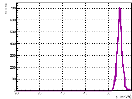
Selected track ST_Foils intersection |p|, foil index 17, N = 4698
