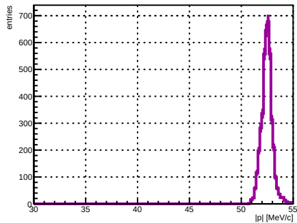
Selected track ST_Foils intersection |p|, foil index 13, N = 4387
