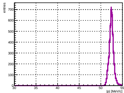
Selected track ST_Foils intersection |p|, foil index 12, N = 4314
