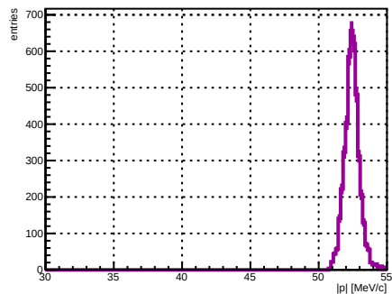
Selected track ST_Foils intersection |p|, foil index 15, N = 4426
