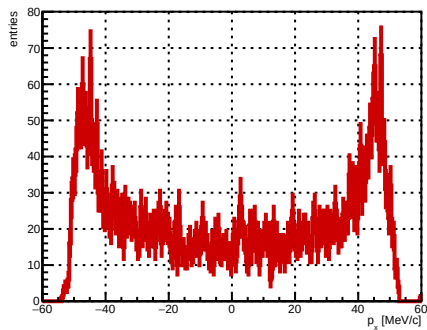
Selected track ST_Foils intersection p_x , foil index 25, N = 4880
