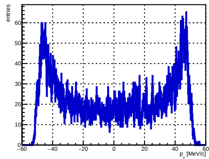
Selected track ST_Foils intersection p_y , foil index 32, N = 4920
