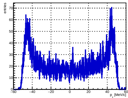
Selected track ST_Foils intersection p_y , foil index 35, N = 4836
