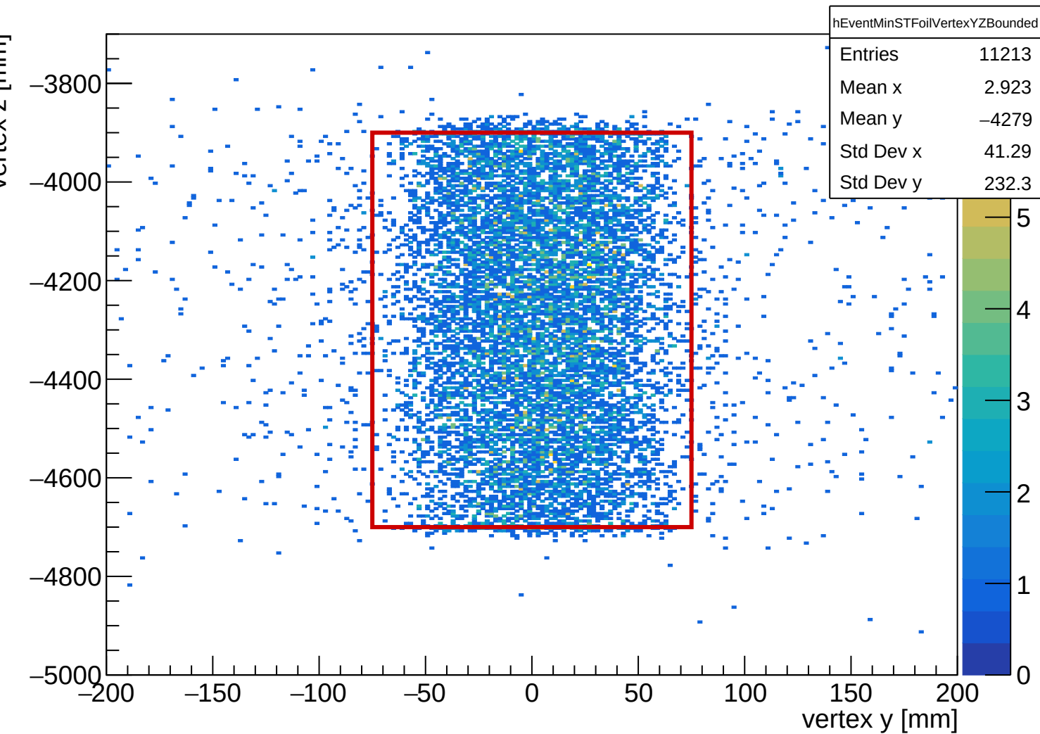
Bounded: event-level closest shared ST_Foils midpoint vertex YZ
