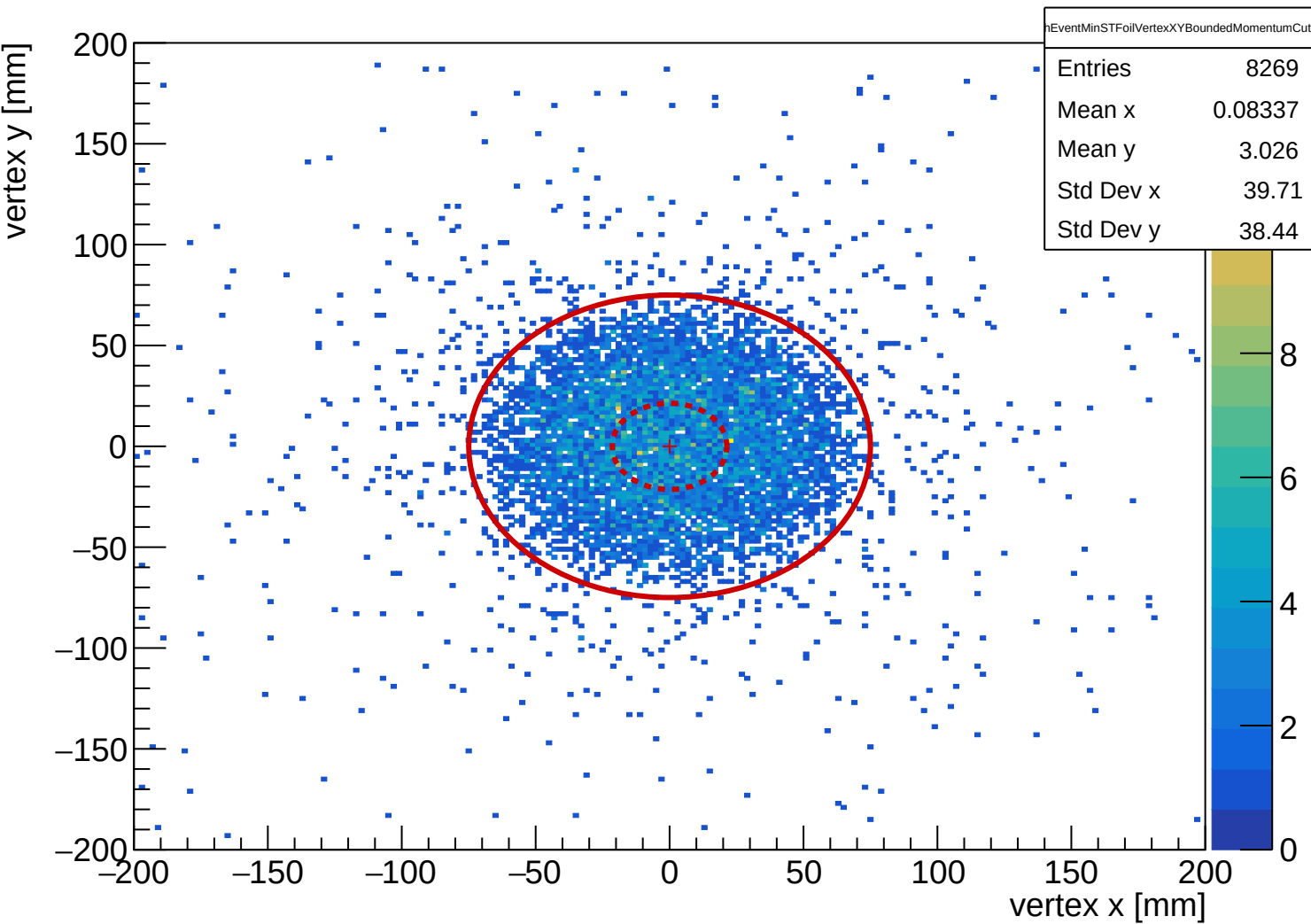
Bounded: Momentum cut: event-level closest shared ST_Foils midpoint vertex XY
