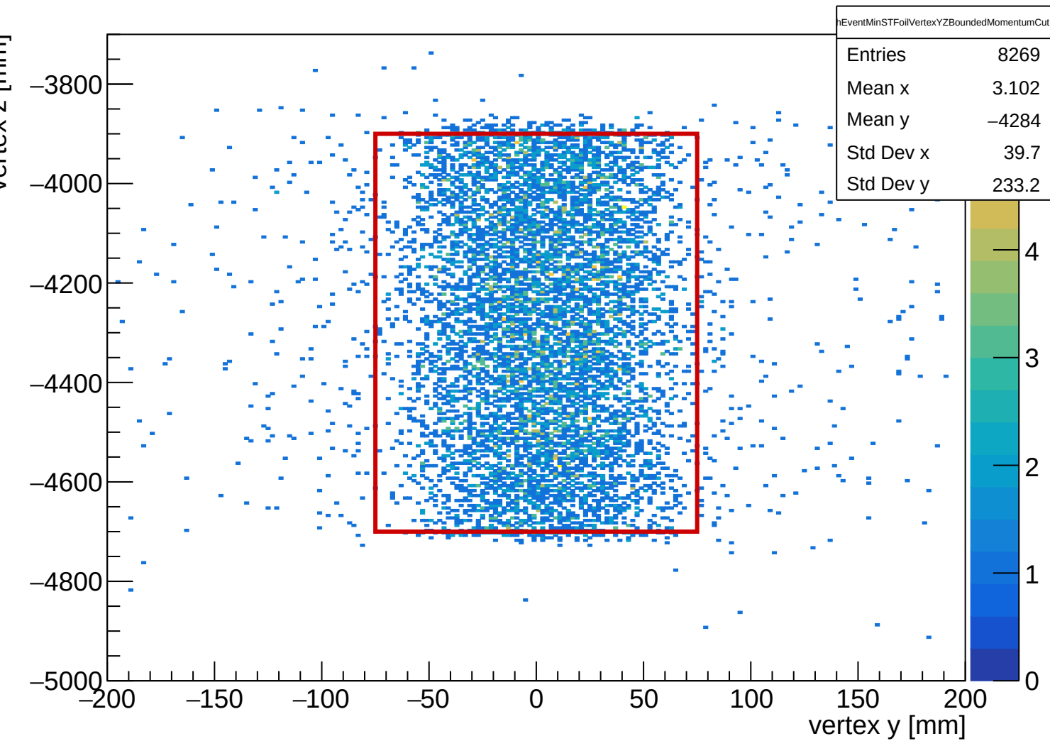
Bounded: Momentum cut: event-level closest shared ST_Foils midpoint vertex YZ
