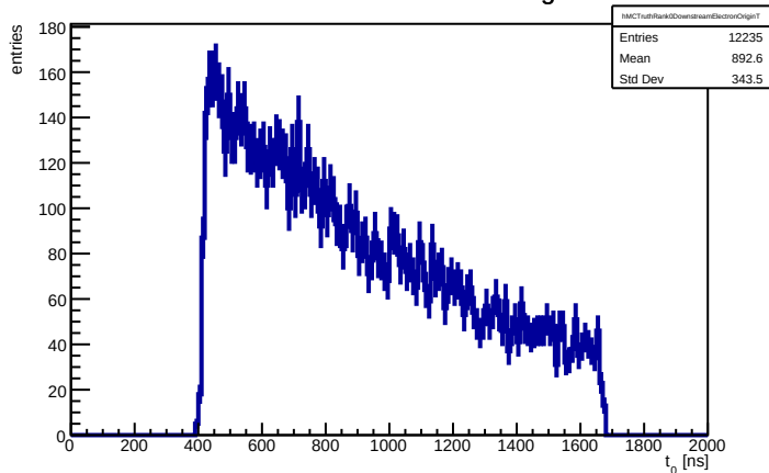
MC truth rank-0 downstream e^- origin time
