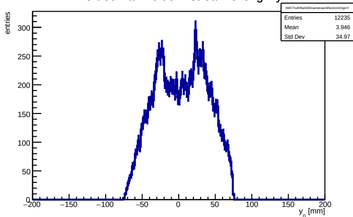
MC truth rank-0 downstream e^- origin y
