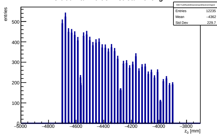
MC truth rank-0 downstream e^- origin z
