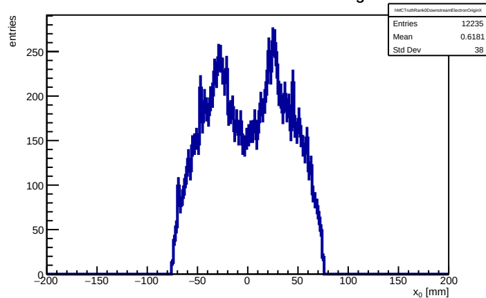
MC truth rank-0 downstream e^- origin x
